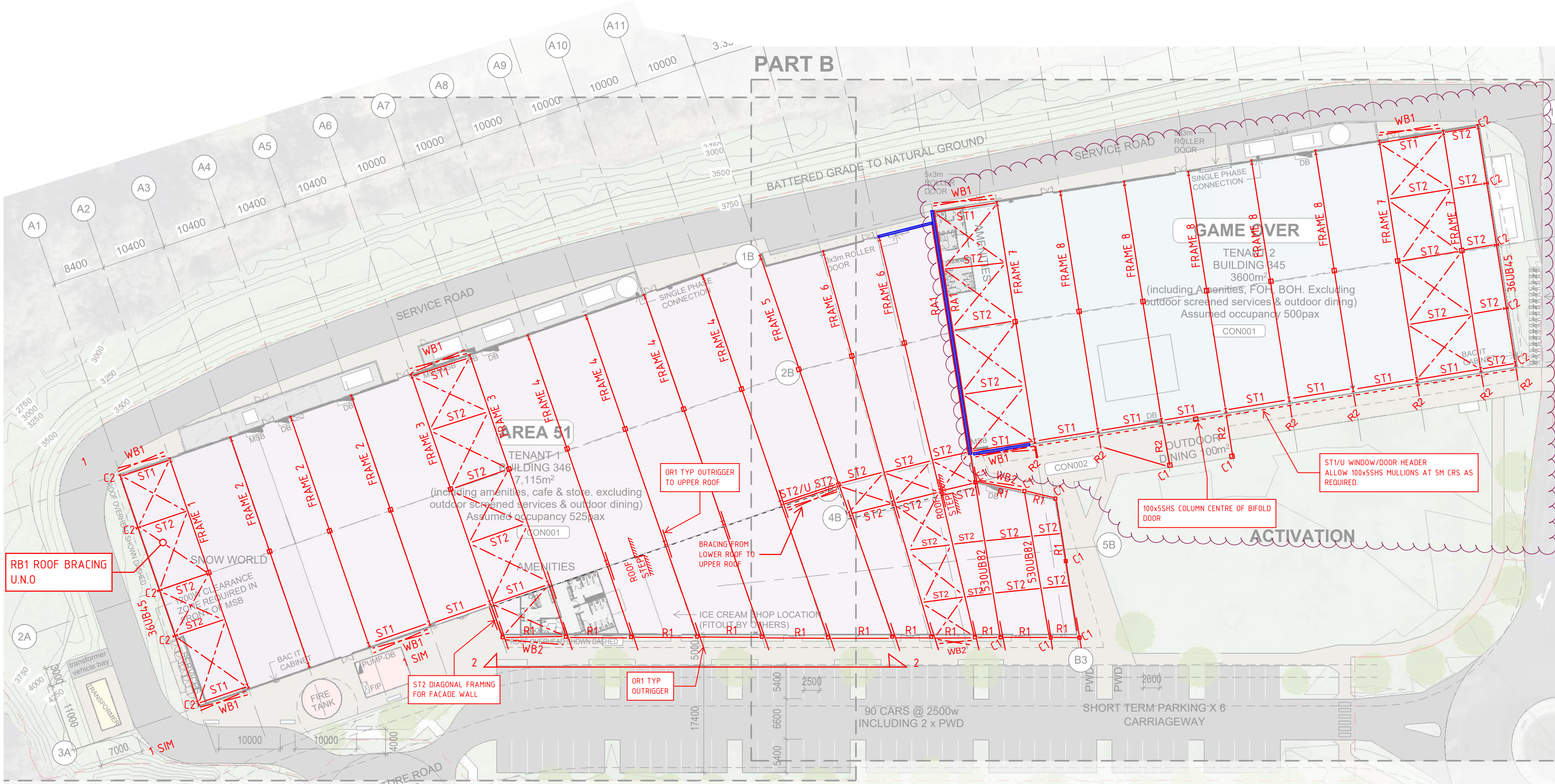
ROOF FRAMING PLAN
